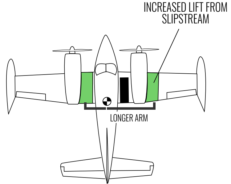
ACCELERATED SLIPSTREAM
