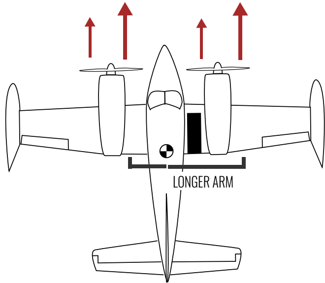
P-FACTOR
