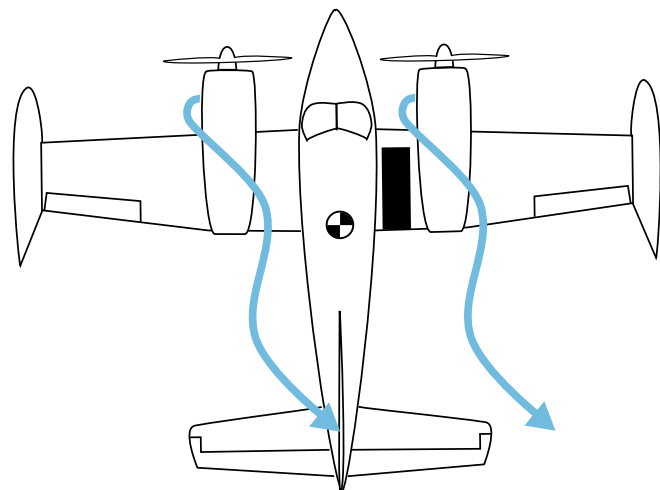
SPIRALING SLIPSTREAM
